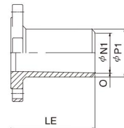
MODEL 904 Extended Butt Weld End
